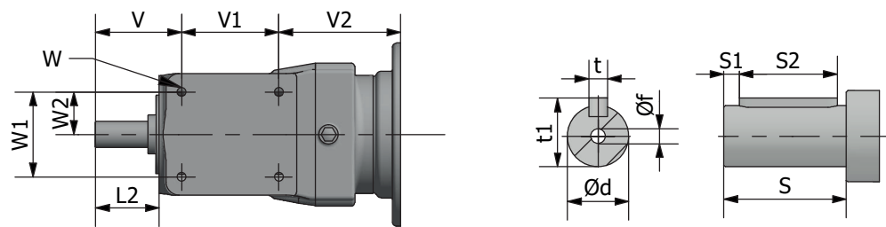
Shaft
