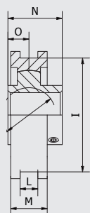
Stainless Steel UC insert , with grub screw
