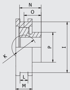
Stainless Steel SA insert, with eccentric ring
